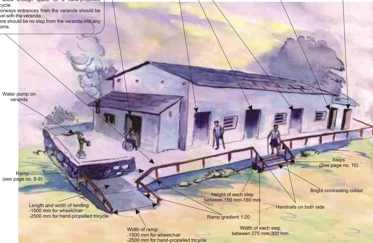
Example of emergency shelter in hill and mountain areas
