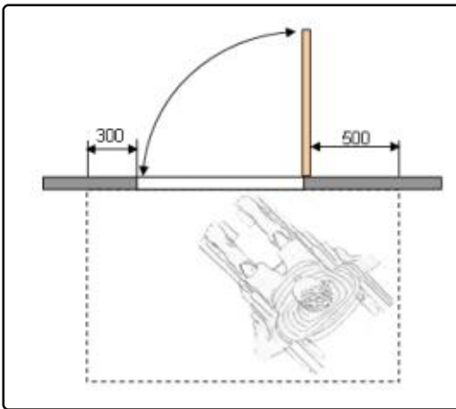
Entrances with sufficient space to maneuver
